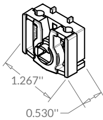
Universal shoe "Supa-lock" G1-42-SL40-00
